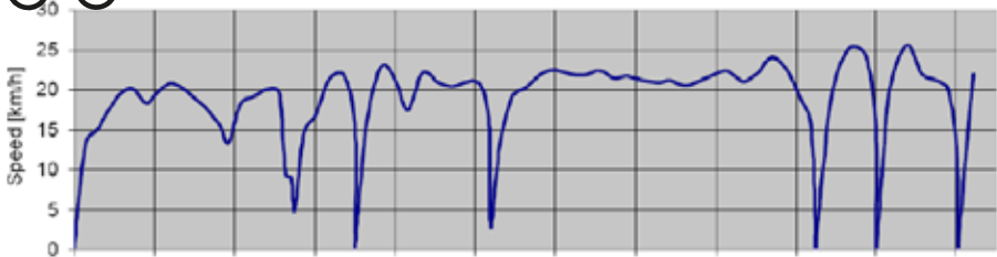
Speed profile - Nørrebrogade - bicycle (After green wave)
